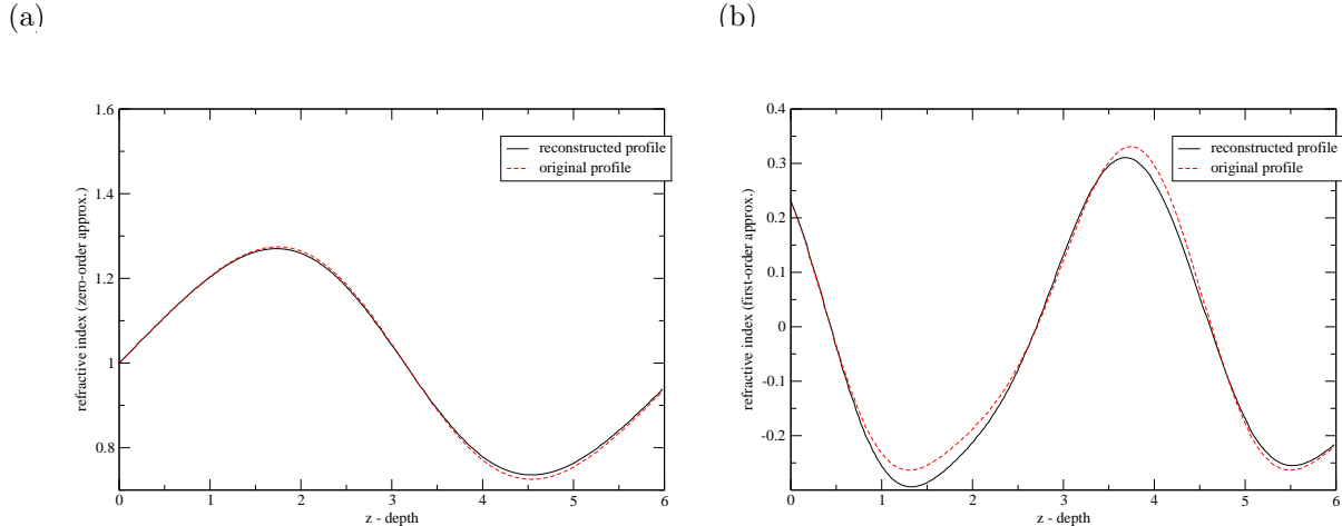
Figure 1: Numerical values of the refractive index n_0 - (a) and n_1 - (b) against original profile (The first group of data with \delta y = 0.08 ).
