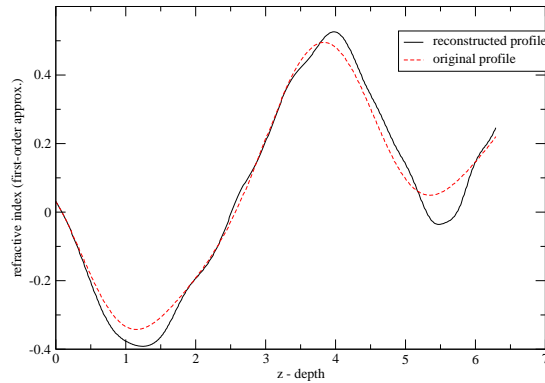
Figure 2: Numerical values of the refractive index n_0 with \delta y = 0.08 - (a) and with \delta y = 0.02 - (b) as well as n_1 with \delta y = 0.02 - (c) against original profile (The second group of data).
